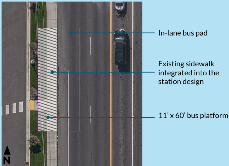
Draft station drawing - design in progress
